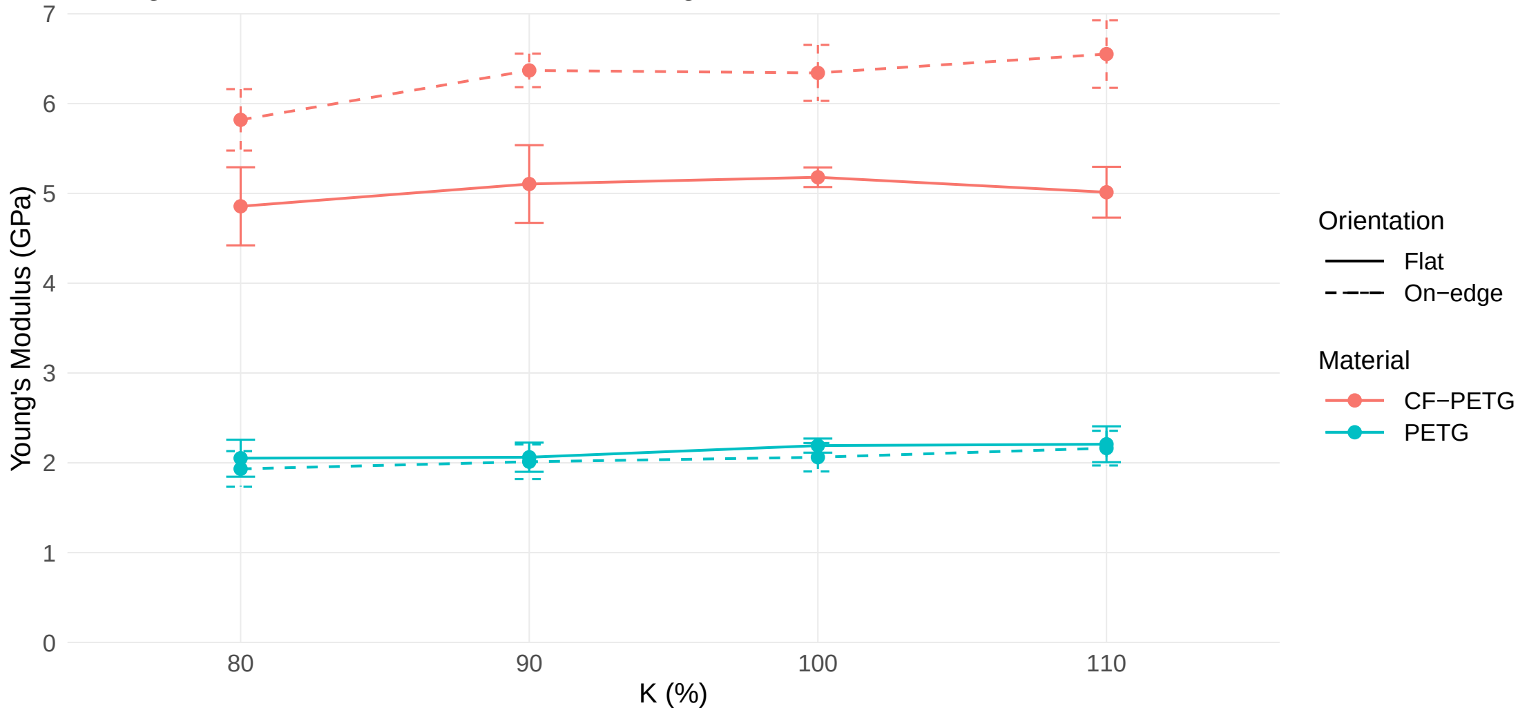
Young's Modulus vs K — Flat vs On-edge Orientation
